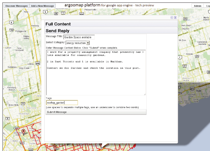
Authoring functionality in Argoomap-GAE. (See page 145 / voir 145)
